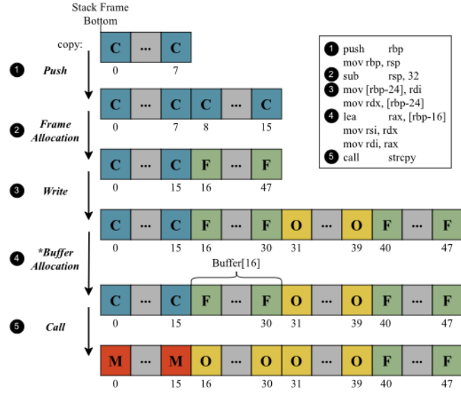
Fig. 8. Example of the MemStaCe for the copy function in Listing 2, where C: Critical, O: Occupied, F: Free, M: Modified.
