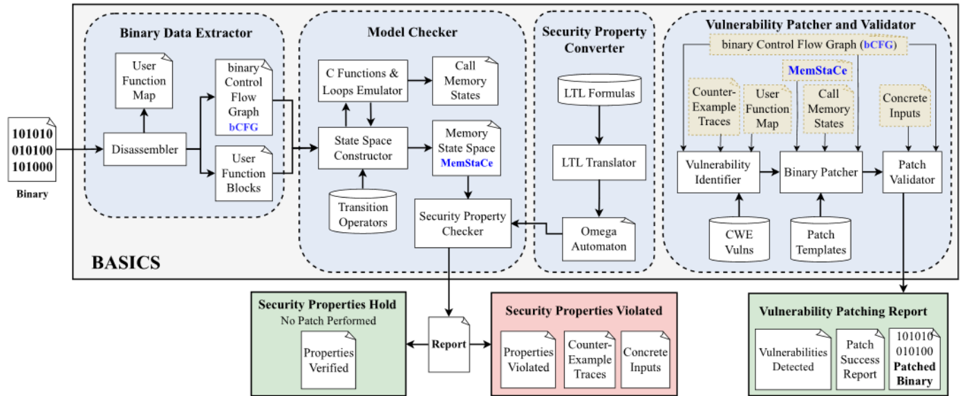
Fig. 1. Overview of the proposed BASICS's approach.
